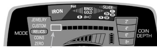
In RELICS Mode, the lowest 2 ferrous pixels are notched out.
